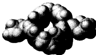
Fig. 2. Crystal structure of 14a . (NO 3 - omitted.)
