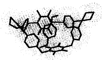
Fig. 4. An MM2 (CACHe, ver. 3.5) optimized structure of the 16a-17 complex.
