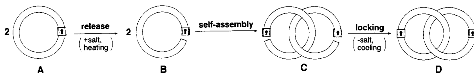
Fig. 7. Schematic presentation of the procedure for the irreversible formation of a catenane from two complete rings using the molecular lock.
